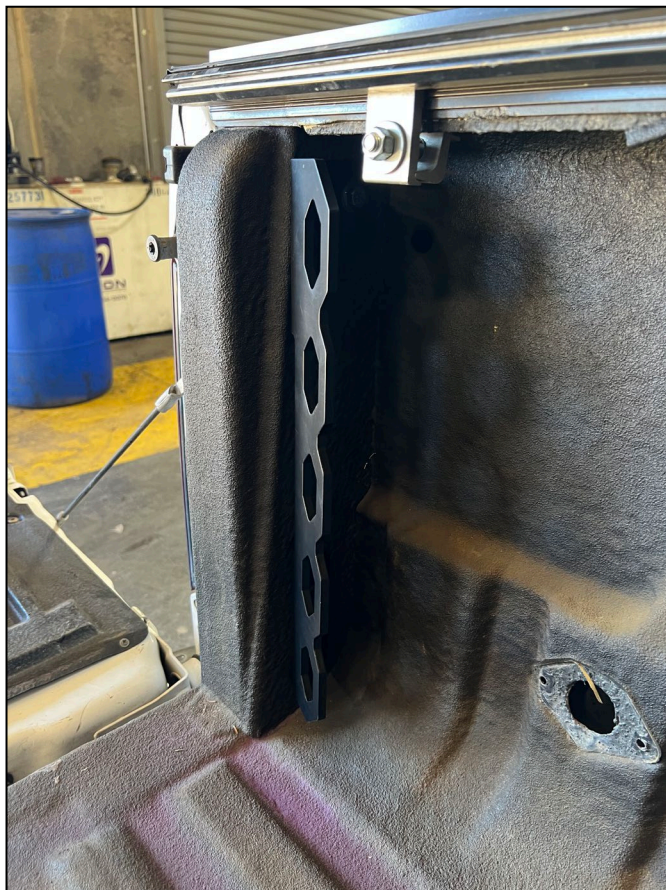
6. Driver Side Tie Down Mounted
