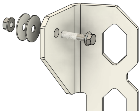
5. Top Hardware Installed (both washers same side)
